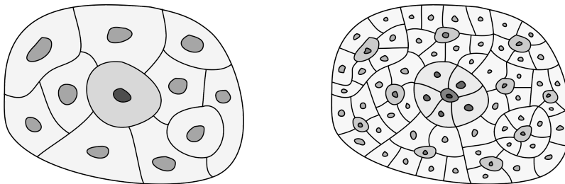
FIGURE 8.2. Possible densities f_0 f_1|_Q (left) and f_0 f_1 f_2|_Q (right).
