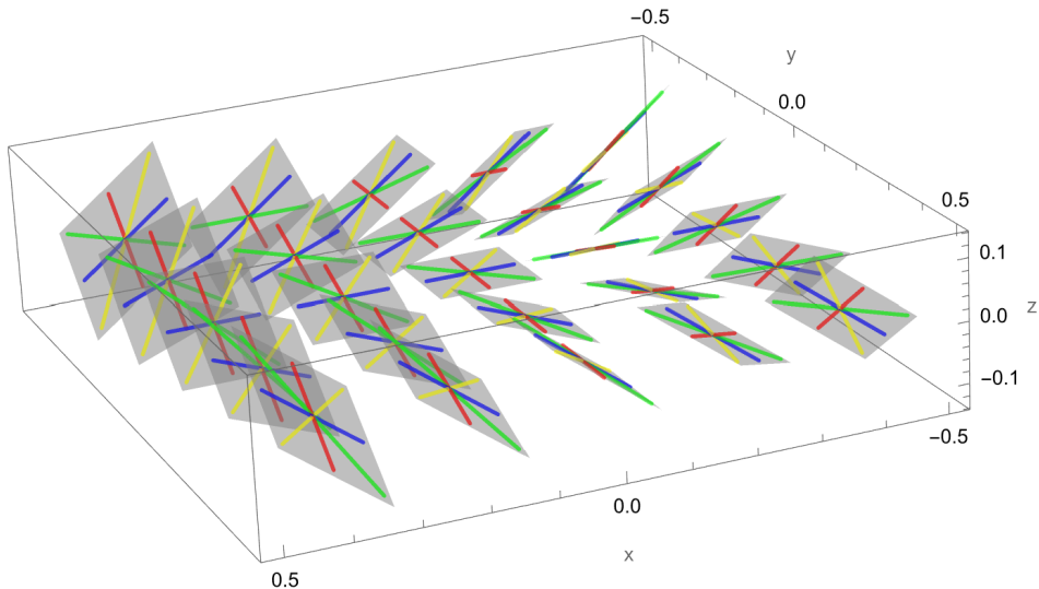
FIGURE 1.2. The simplest example of a nonabelian Carnot group is the first Heisenberg group H^1 , which is topologically equivalent to \mathbb{R}^3 but is equipped with a metric so that H^1 has Hausdorff dimension 4. The step of H^1 is 2. In the illustration, we show 4 horizontal line segments at 25 points located in the xy -plane inside of H^1 .
