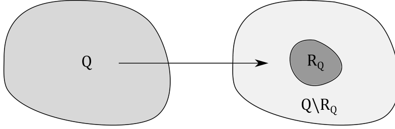
FIGURE 8.1. To define f_Q d\mu , redistribute the mass \mu(Q) so that more mass is assigned to R_Q and less mass is assigned to Q \setminus R_Q .
