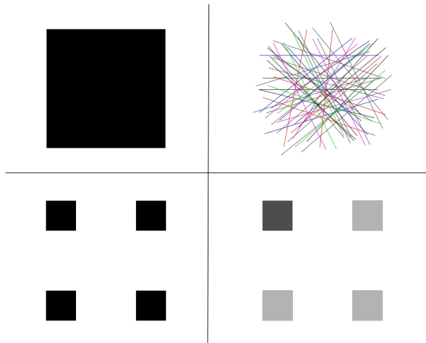
FIGURE 1.1. The 2-dimensional Lebesgue measure \mathcal{L}^2 in the plane \mathbb{R}^2 is purely 1-unrectifiable (top left). A countable sum \mu = \sum_i^\infty \mu_i of measures \mu_i supported on line segments I_i is a 1-rectifiable measure with support \overline{\bigcup_i I_i} (top right); in particular, there are examples of this type with \text{spt } \mu = \mathbb{R}^2 . The natural Hausdorff measure \mathcal{H}^s \llcorner E_s restricted to a Cantor set E_s of Hausdorff dimension s is 1-rectifiable when s < 1 and purely 1-unrectifiable when s \geq 1 (bottom left). A self-similar measure \mu supported on the set E_1 is 1-rectifiable when the generating sets for E_1 have unbalanced weights (bottom right). This illustrates that it is possible for a rectifiable measure to have purely unrectifiable support.
